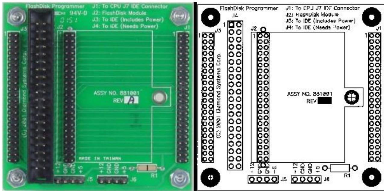
FlashDisk Programmer Board Layout
