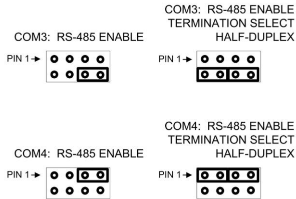
J18 Jumper Block
