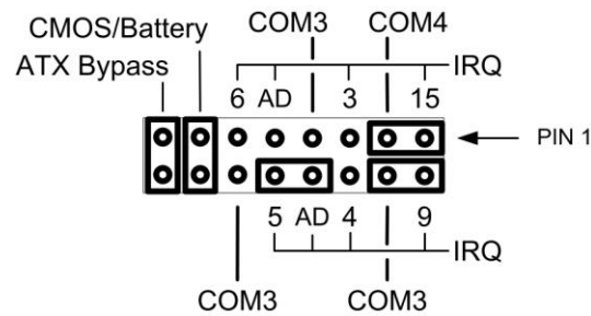
J10 Jumper Block with Default Settings
