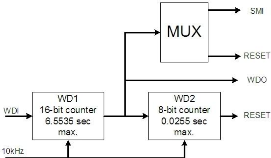
Watchdog Timer Block Diagram
