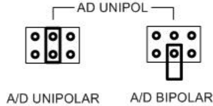
A/D Unipolar/Bipolar Selection
