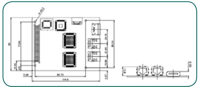
e-SATA Connector
