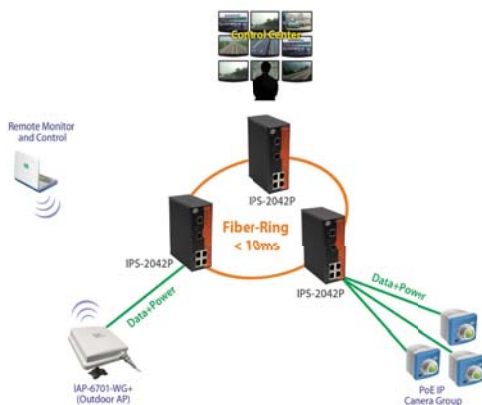
Network connection
