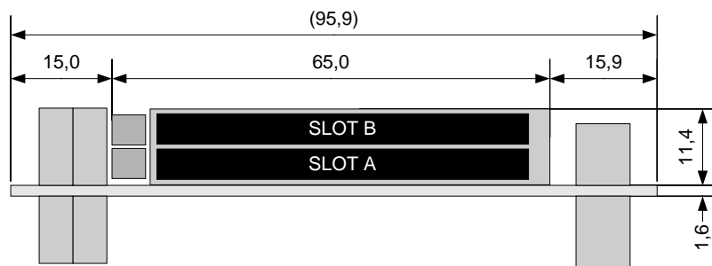
Figure 10: PCCard-x Side View
