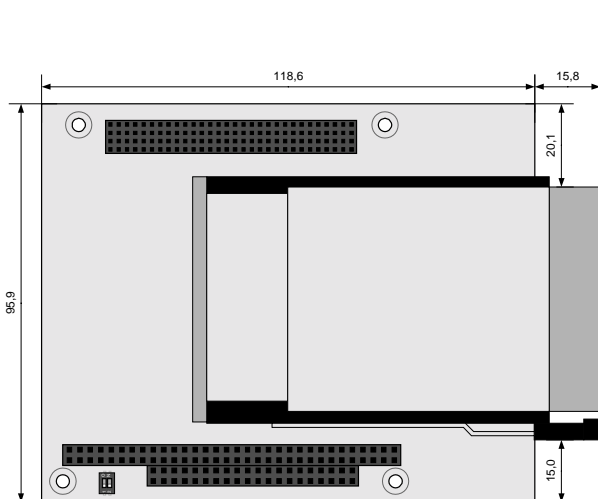
Figure 8: PCCard-M
