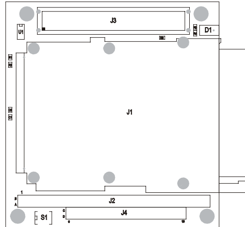
Figure 2: PCCard-P For A PC104+ System
