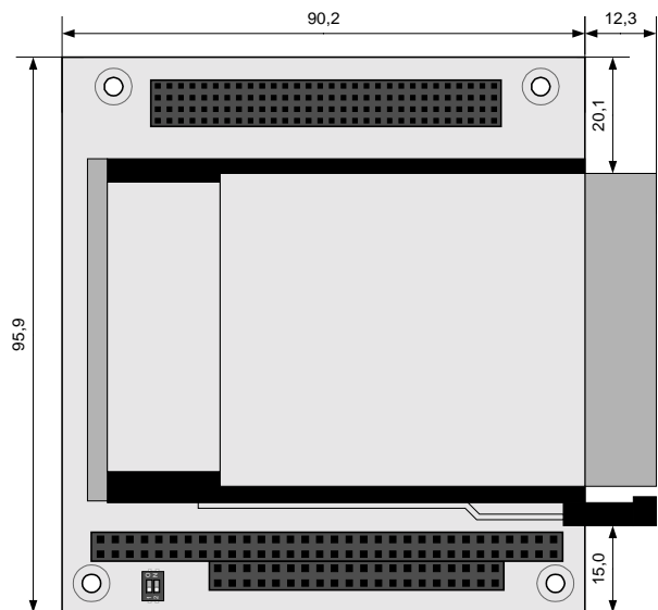
Figure 9: PCCard-P
